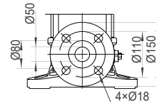
Flange PN25/DN40
