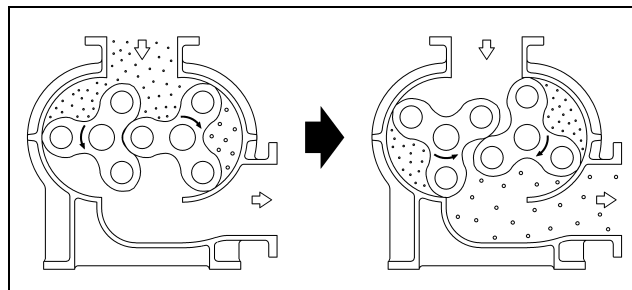
Rotor 3 cam Three-Lobed Rotor
