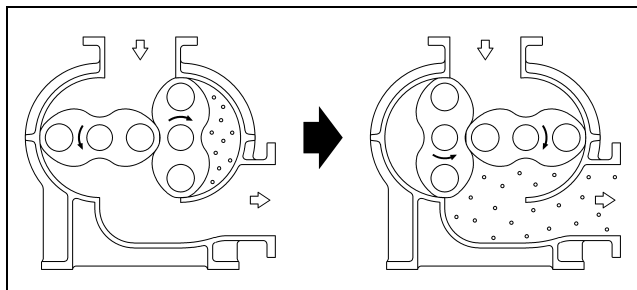
Rotor 2 cam Two-Lobed Rotor
